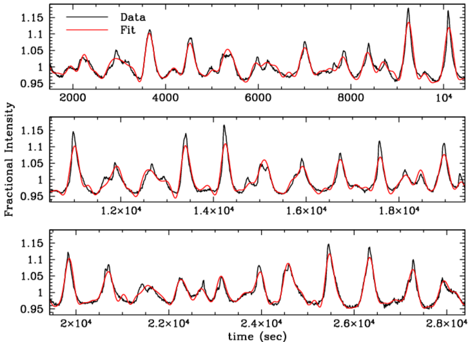
Fit to not_09_lc.dat
